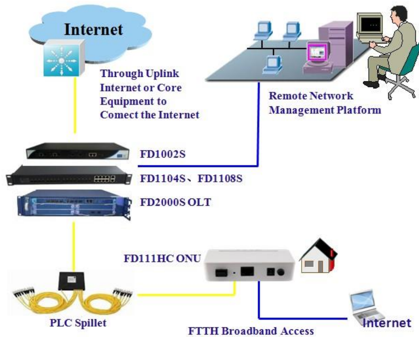
Figure: APFD111HZ Application Diagram
